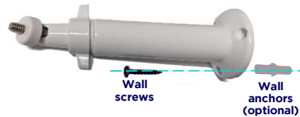
Figure 2: Mounting the bracket with screws and optional wall anchors
