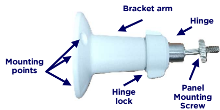
Figure 1: Mounting bracket parts
