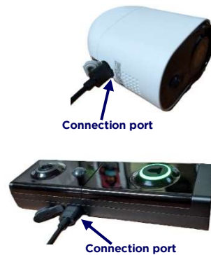
Figure 4: Connecting to Outdoor Camera and Wireless Doorbell
