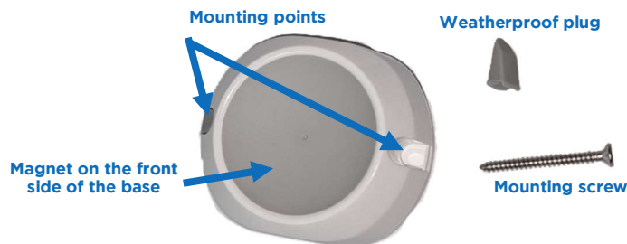
Figure 3: Mounting screw points and weatherproofing plugs
